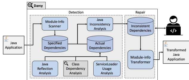
Fig. 2: A high-level overview of DARC Y
