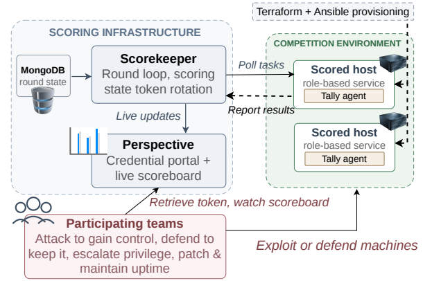
Figure 2: The Netsiege toolchain and its interaction with the competition environment and teams.
