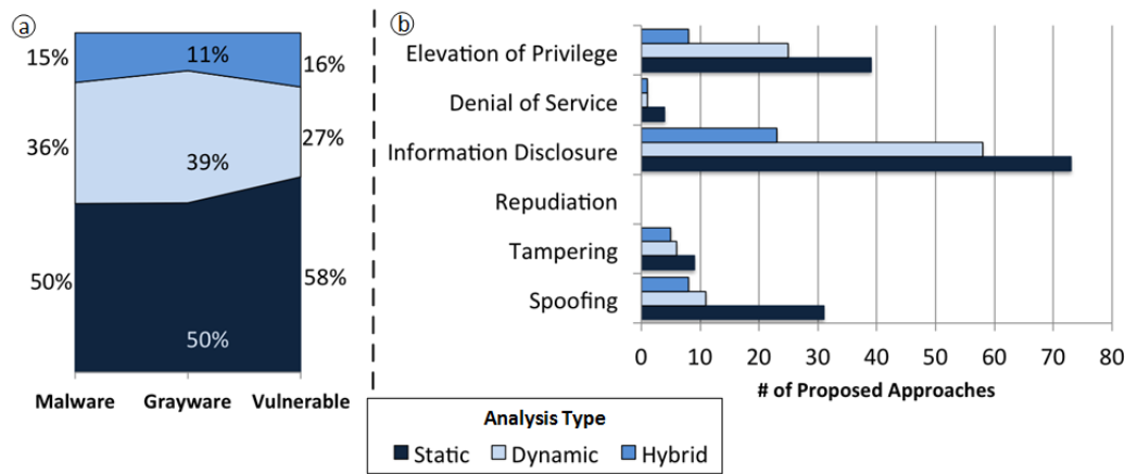
Fig. 14. Types of program analysis that have been used for detecting (a) different security assessment objectives (i.e. malware vs. vulnerability detection), and (b) different security threats.
