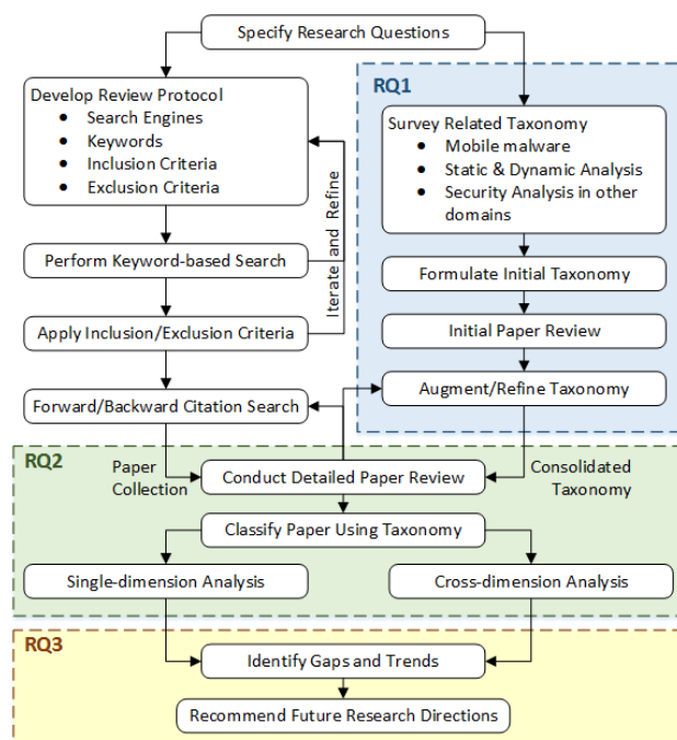
Fig. 1. Research process flow and tasks.
