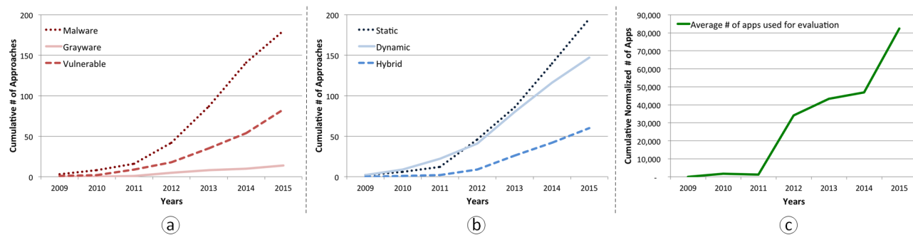
Fig. 18. Observed trends in Android security analysis research with respect to (a) objectives of the analysis, (b) type of analysis, and (c) number of apps used in the evaluation (normalized by dividing the number of apps to the number of publications in each year).
